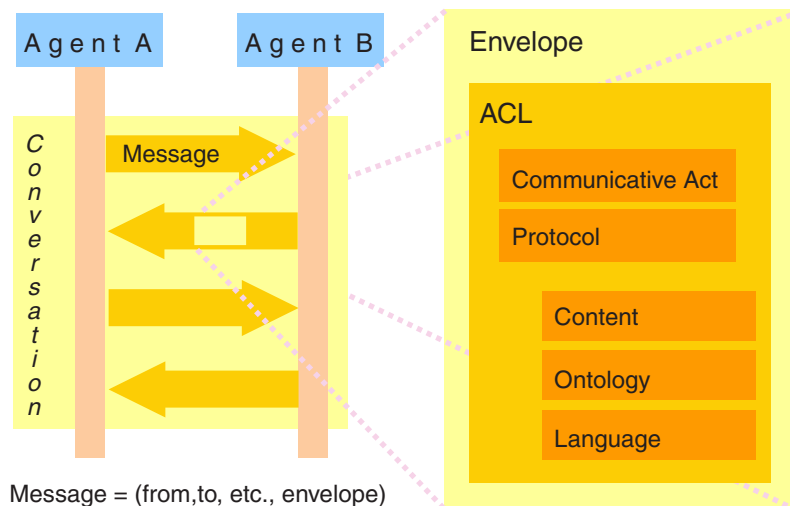
Figure 6: FIPA Agent Communication
